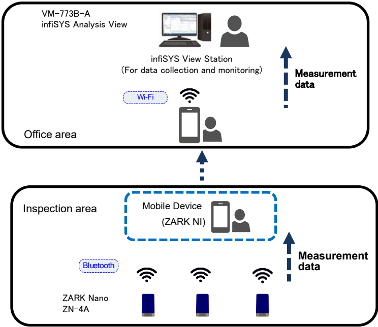
Figure 1 Example of system configuration
